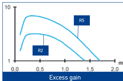
Excess gain
