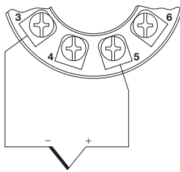
Thermocouple with internal cold junction compensation
