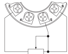
Potentiometer, 3-wire
