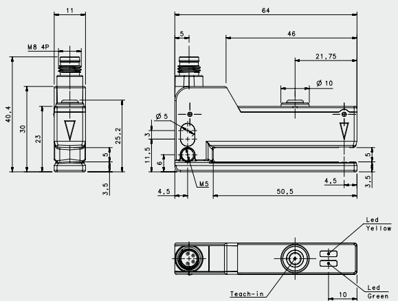
M8 CONNECTOR
