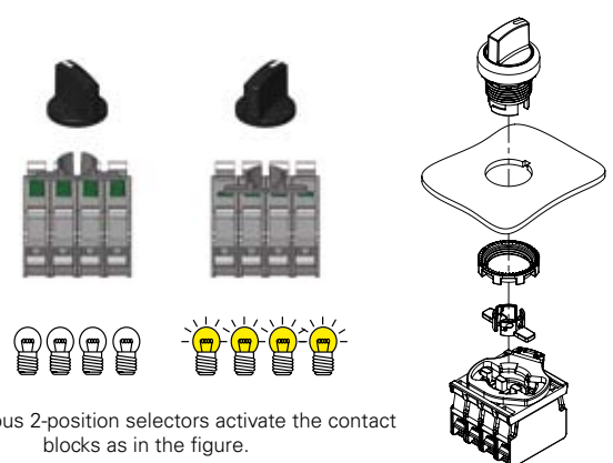
Fixing adapter with 4 positions
