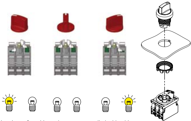
Fixing adapter with 3 positions
