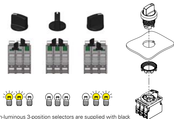
Fixing adapter with 3 positions
