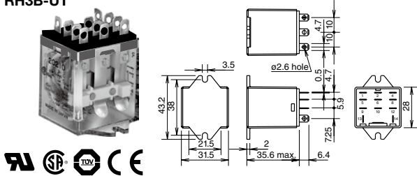
3PDT Plug-in Terminal (Top Bracket Mounting) RH3B-UT
